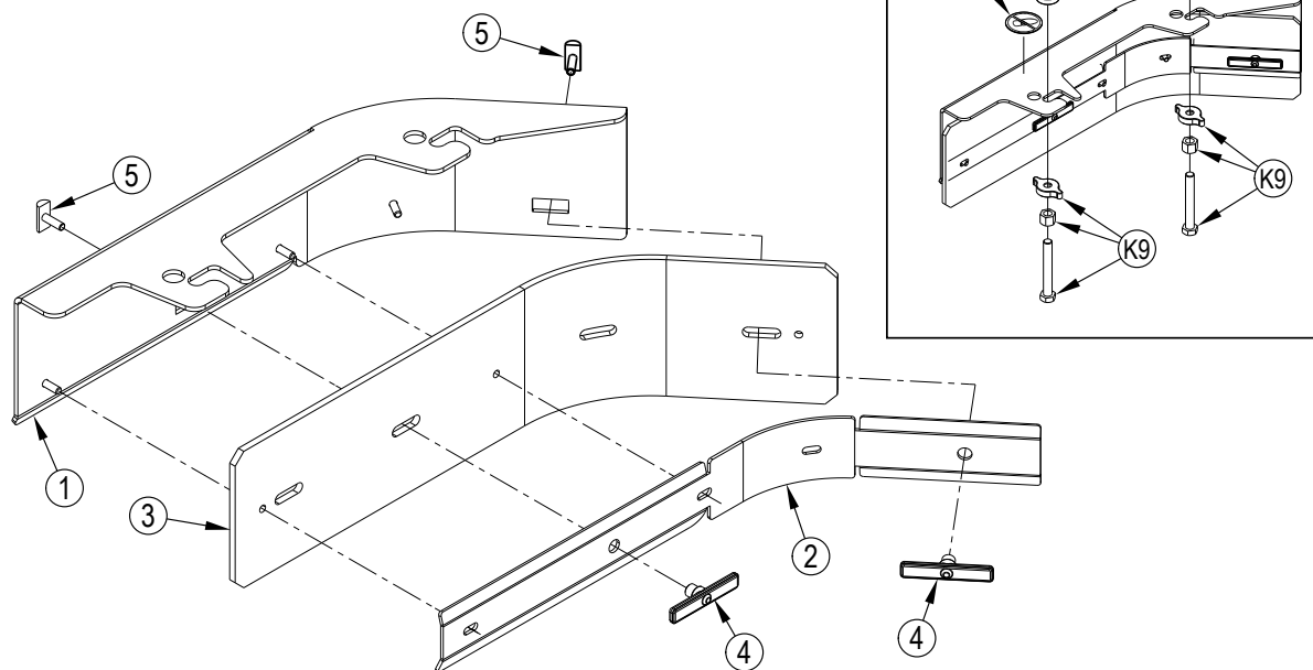
RIGHT SIDE SKIRT ASSEMBLY 860D
