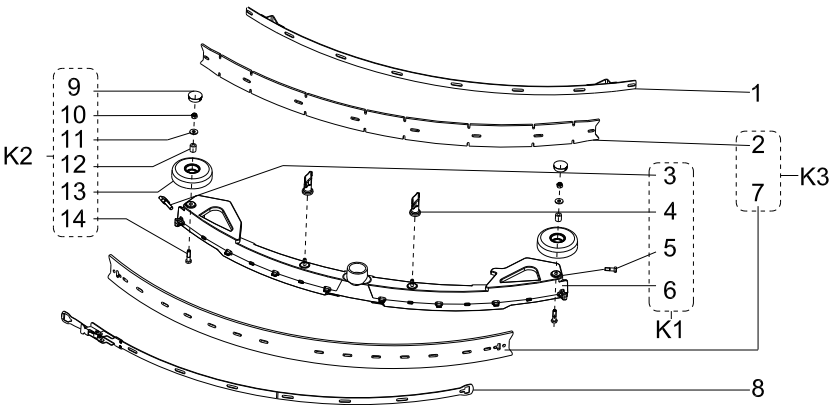
SQUEEGEE ASSEMBLY BR755 ,559504340
